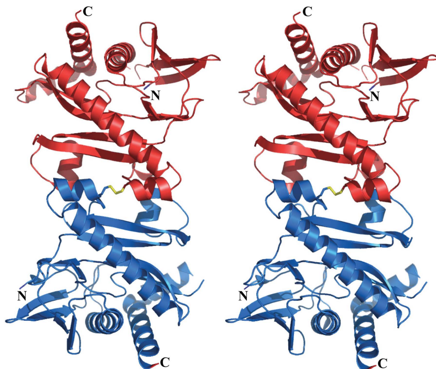
Figure 3 Dimeric SAICAR synthase. The covalent dimer is pictured here in stereo with one peptide chain in red and the other in blue. The amino-termini are labeled N and the carboxy-termini are labeled C. The disulfide bridge is located across a (noncrystallographic) twofold axis and is shown as yellow sticks.
