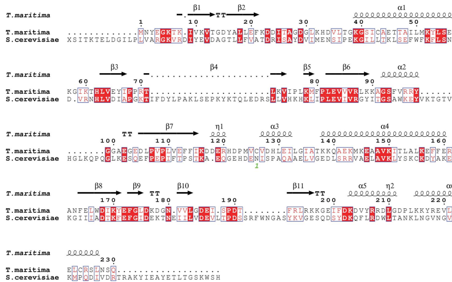
Figure 2 Structure-based primary sequence alignment of SAICAR synthases from T. maritima and baker's yeast ( S. cerevisia ). Identical residues are highlighted and secondary-structure motifs are labeled above: \beta -strands are depicted as arrows and \alpha -helices as coils. The numbering is that for the T. maritima enzyme. This figure was generated using the ESPrInt utility (Gouet et al. , 1999).
